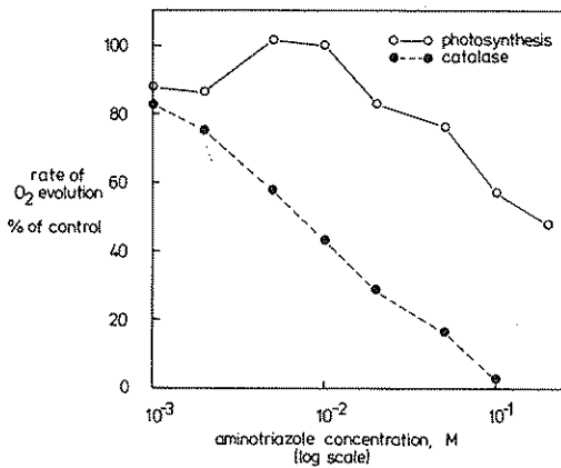
FIG. 3. Inhibition by aminotriazole of photosynthetic O_2 evolution ( CO_2 -dependent) and of catalase in the chloroplast preparation; Chl concentration was 20 \mu g \text{ ml}^{-1} . Photosynthetic O_2 evolution: chloroplasts 59% intact; control rate: 35 \mu \text{mol of } O_2 \text{ (mg of Chl)}^{-1} \text{ hr}^{-1} ; catalase activity of chloroplast preparation: 10 units ( \text{mg of Chl}^{-1} ). Catalase activity: chloroplasts 40% intact; control activity: 13 units ( \text{mg of Chl}^{-1} ).
