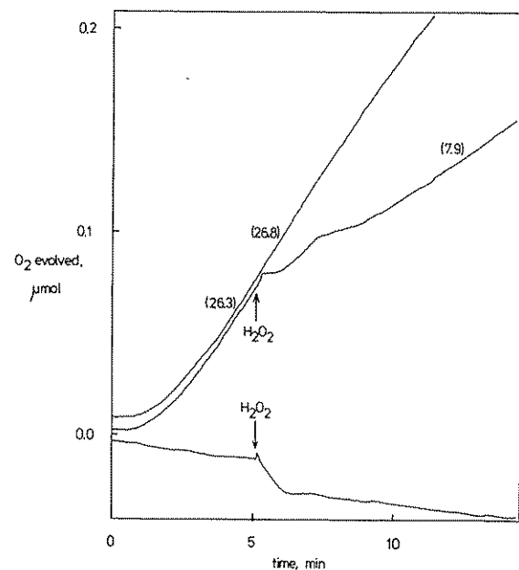
FIG. 5. O_2 electrode trace showing effect of H_2O_2 ( 0.4 \mu \text{mol} ) on CO_2 -dependent O_2 evolution by isolated chloroplasts in the presence of aminotriazole (50 mM). Middle trace shows this effect of H_2O_2 . Lower trace is a dark control; upper trace is of an illuminated reaction to which no addition of H_2O_2 was made. Bracketed figures are rates of O_2 evolution in \mu \text{mol of } O_2 \text{ (mg of Chl)}^{-1} \text{ hr}^{-1} . Chloroplasts 50% intact.
