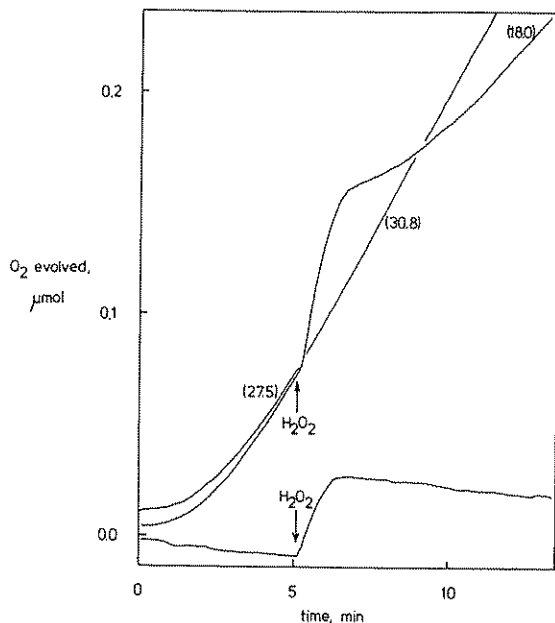
FIG. 4. O_2 electrode trace showing effect of H_2O_2 ( 0.4 \mu \text{mol} ) on CO_2 -dependent O_2 evolution by isolated chloroplasts. Middle trace shows this effect of H_2O_2 . Lower trace is a dark control, and the upper trace is that of an illuminated reaction to which no addition of H_2O_2 was made. Bracketed figures are rates of O_2 evolution in \mu \text{mol of } O_2 \text{ (mg of Chl)}^{-1} \text{ hr}^{-1} . Chloroplasts 50% intact.
