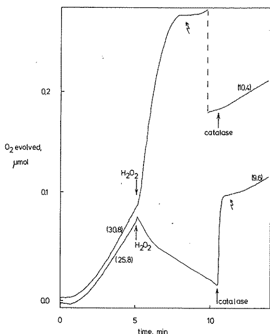
FIG. 6. Effect of \text{H}_2\text{O}_2 ( 0.8 \mu\text{mol} ) on \text{CO}_2 -dependent \text{O}_2 evolution by chloroplasts in the absence of a catalase inhibitor (upper trace) and in the presence of 50 \text{ mM} aminotriazole (lower trace). Vertical broken line indicates adjustment of zero position on chart recorder. Bracketed figures are rates of \text{O}_2 evolution in \mu\text{mol of O}_2 (\text{mg of Chl})^{-1} \text{ hr}^{-1} . Catalase added: 5 \times 10^3 units. Chloroplasts 50% intact. Offset arrows ( \xi ) indicate resumption of photosynthetic \text{CO}_2 -dependent \text{O}_2 evolution after \text{H}_2\text{O}_2 treatment.
