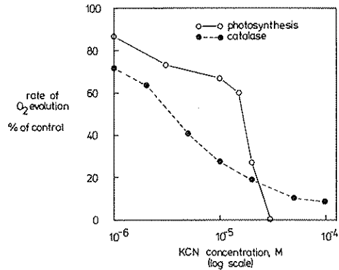
FIG. 1. Inhibition by KCN of photosynthetic O 2 evolution (CO 2 -dependent) and of catalase in chloroplast preparations; Chl concentration was 20 μg ml -1 . Photosynthetic O 2 evolution: chloroplasts 58% intact; control rate was 25 μmol O 2 (mg Chl) -1 ; unshocked chloroplast preparation had a catalase activity of 10 units (mg of Chl) -1 . Catalase activity: chloroplasts 40% intact; control activity: 13 units (mg of Chl) -1 .
